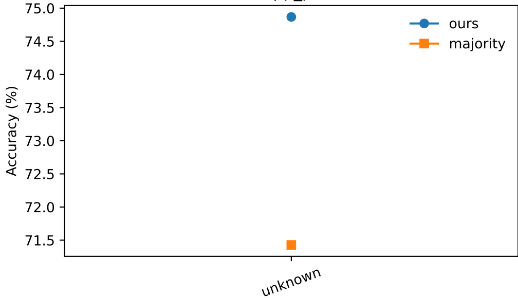
mbpp_plus
