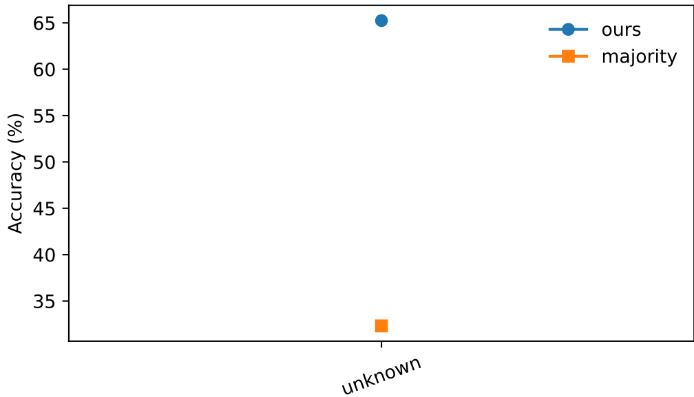
humaneval_plus
