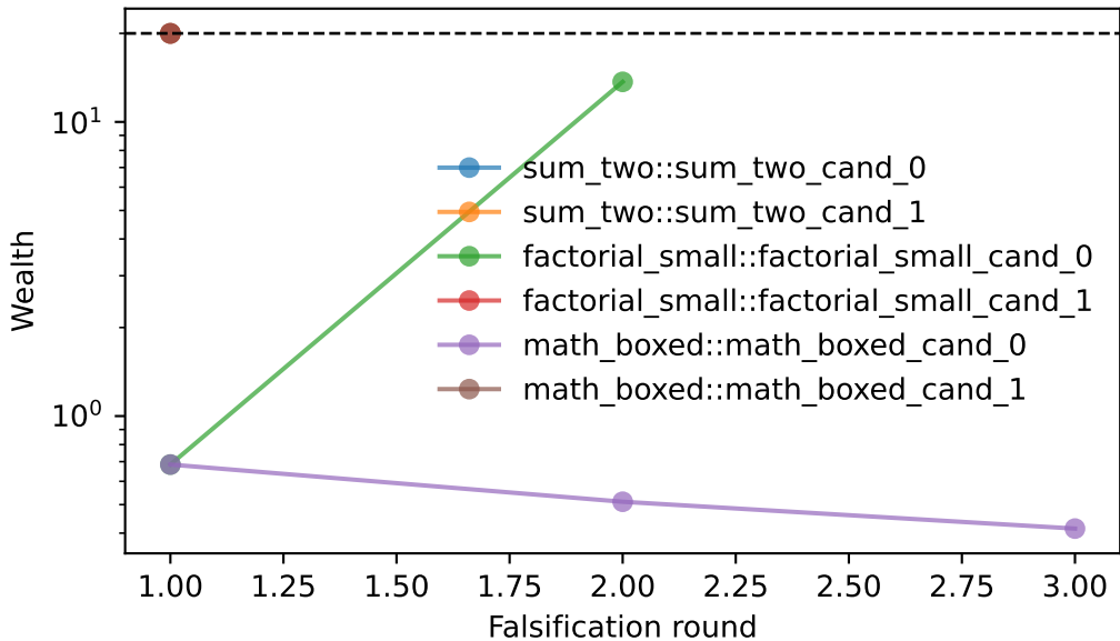
E-value Wealth Process
