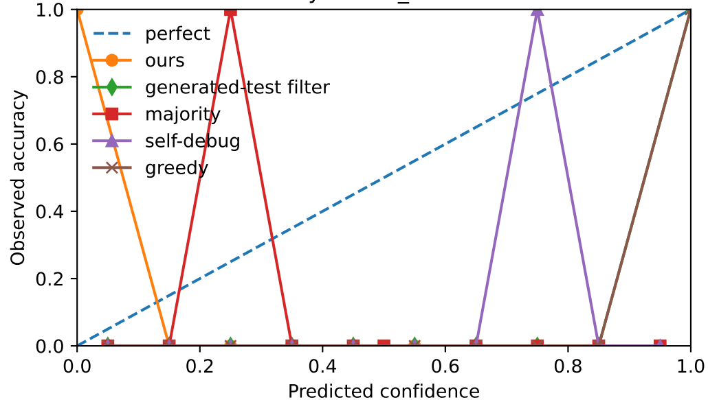
synthetic_demo
