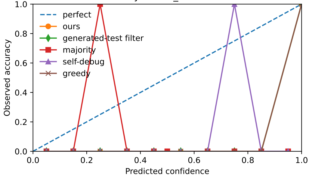
synthetic_demo
