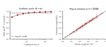
Figure H.9: Oracle convergence. Held-out R^2(\hat{w}, w^*) = 0.998 at n = 2048 .
