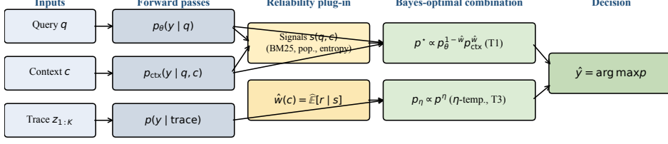
Figure 1: The BAYESARBITER pipeline. Three inputs ( q , c , trace z_{1:K} ) produce three distributions ( p_{\theta} , p_{ctx} , p(\cdot | \text{trace}) ). A reliability plug-in \hat{w}(c) = \hat{\mathbb{E}}[r | s(q, c)] drives the geometric mixture (Section 3.1); the post-trace distribution is \eta -tempered with closed-form Brier improvement (Theorem 4).
