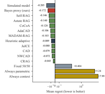
(b) Per-baseline regret (symlog); same ordering visualized.
