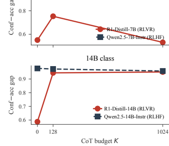
(b) Trace-level RLVR vs. RLHF gap by K .
