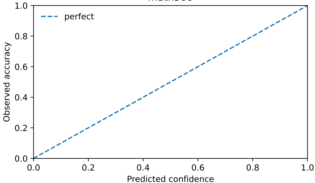
math500
