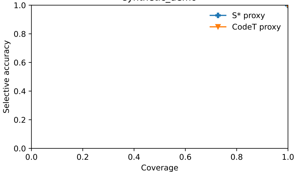
synthetic_demo
