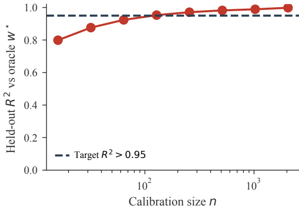
Synthetic oracle: \hat{w} \rightarrow w^*
