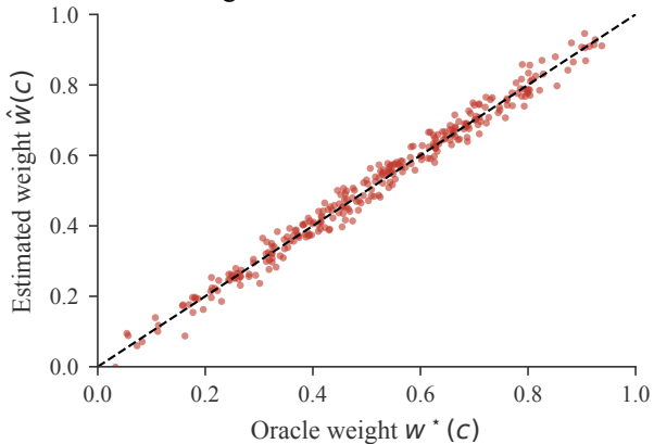
Plug-in estimator at n = 2048
