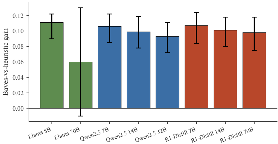
Per-model Bayes-proxy gain (spotlight matrix; mean over 5 benchmarks)
