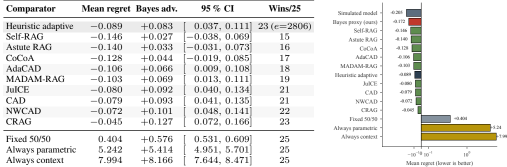
Figure 2: Spotlight comparison against named baselines. Load-bearing comparisons against published methods (Self-RAG, Astute RAG, CoCoA, AdaCAD); heuristic-adaptive is a construction control. 25-cell CIs clear zero against 7 of 10 named methods (heuristic-adaptive at +0.083, plus AdaCAD/MADAM-RAG/JuICE/CAD/NWCAD/CRAG); the three tightest (Self-RAG, Astute, CoCoA) clear zero on the powered n=210 design (Section 4.1) at +0.043/ +0.032/ +0.022.
