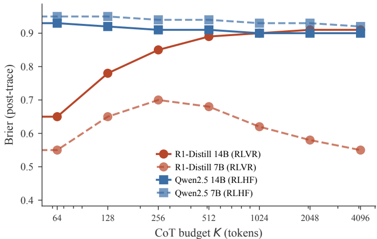
Post-trace Brier vs. K on ConflictBank-conflict
