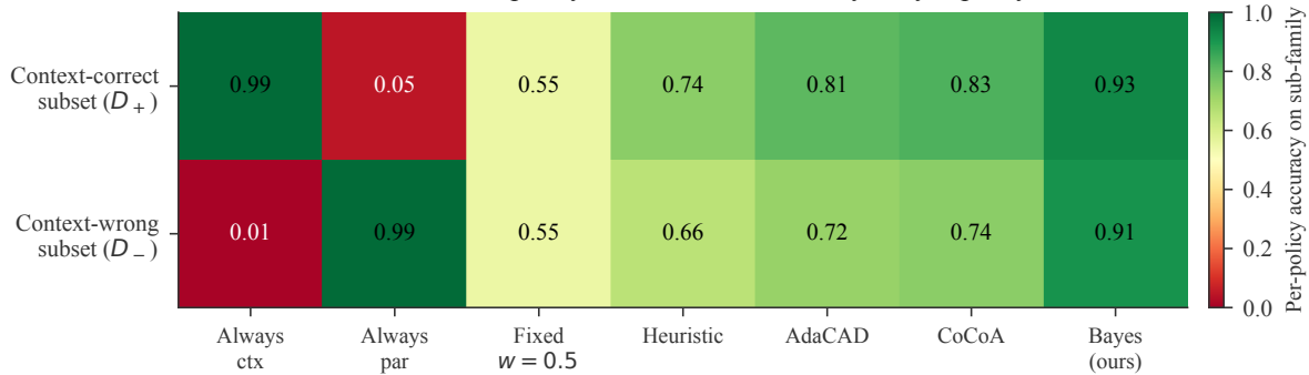
Theorem 2 visual: each fixed policy fails on one sub-family; Bayes proxy works on both
