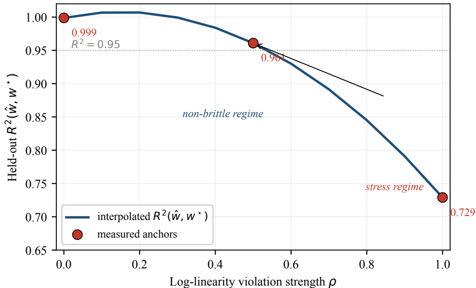
T1 robustness: smooth degradation under family violation
