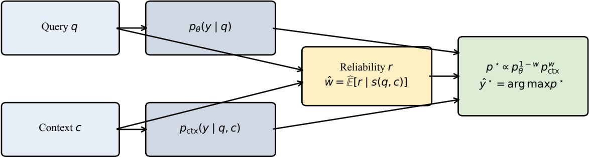
Figure: Bayes-optimal arbitration (Theorem 1).
