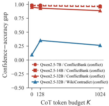
Qwen2.5-Instruct family
