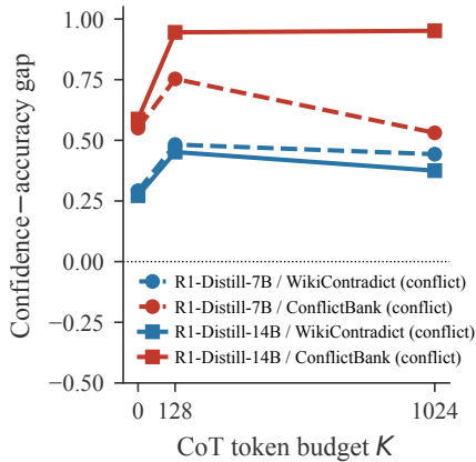
DeepSeek-R1-Distill (RLVR)
