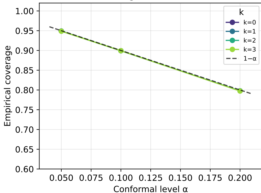
Coverage vs \alpha — MMLU
