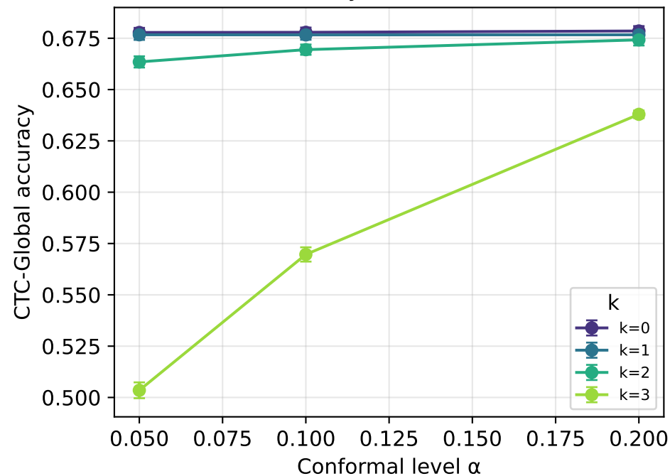
Accuracy vs \alpha — MMLU
