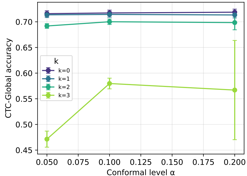
Accuracy vs \alpha — TRUTHFULQA
