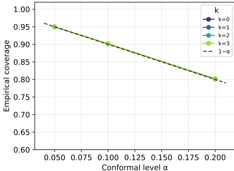
Coverage vs \alpha — TRUTHFULQA
