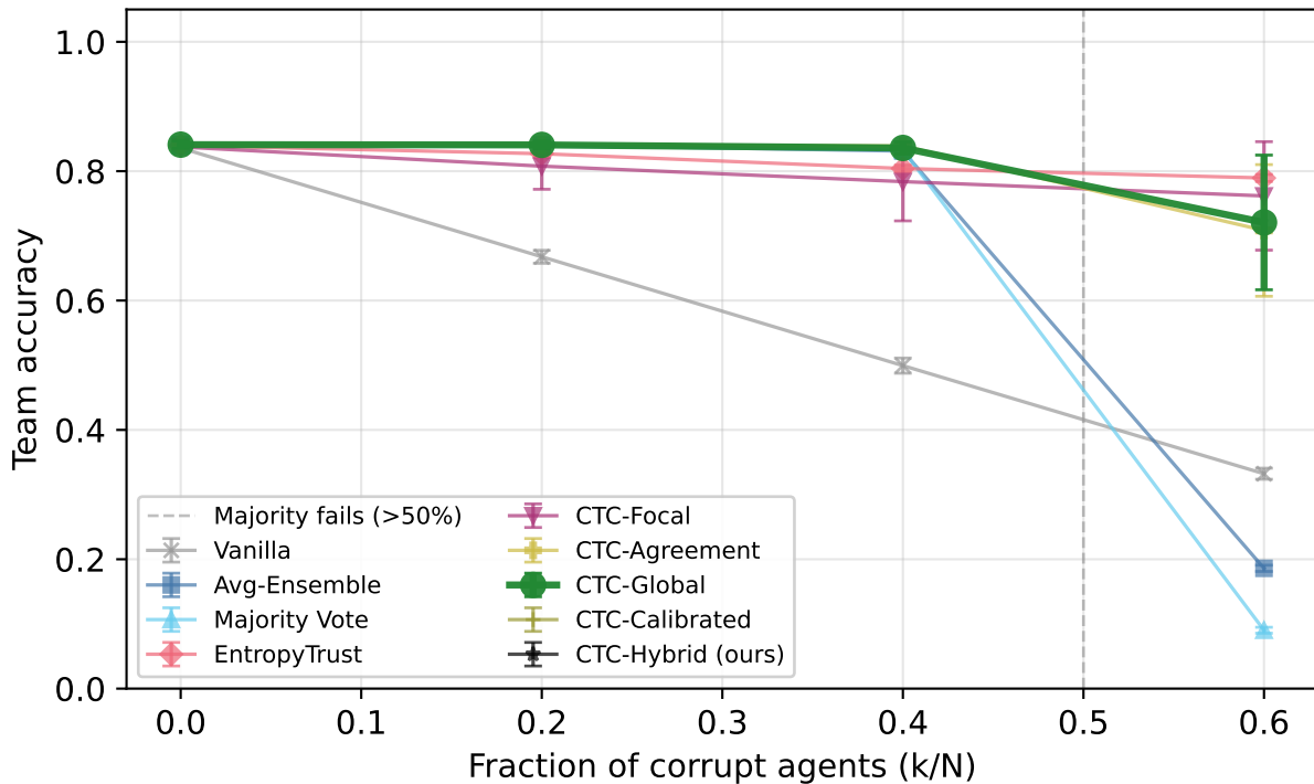
ARC — Phi-3.5-mini-instruct (overconfident, \alpha=0.1 )
