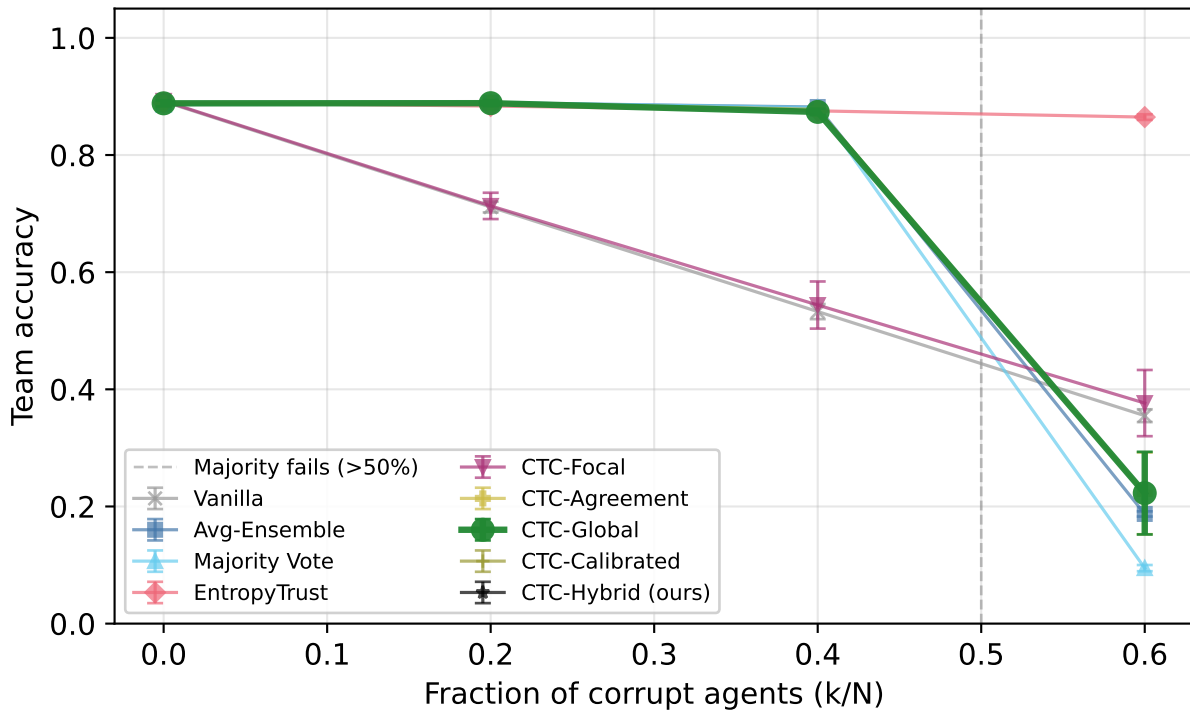
ARC — Qwen2.5-7B-Instruct (overconfident, \alpha=0.1 )
