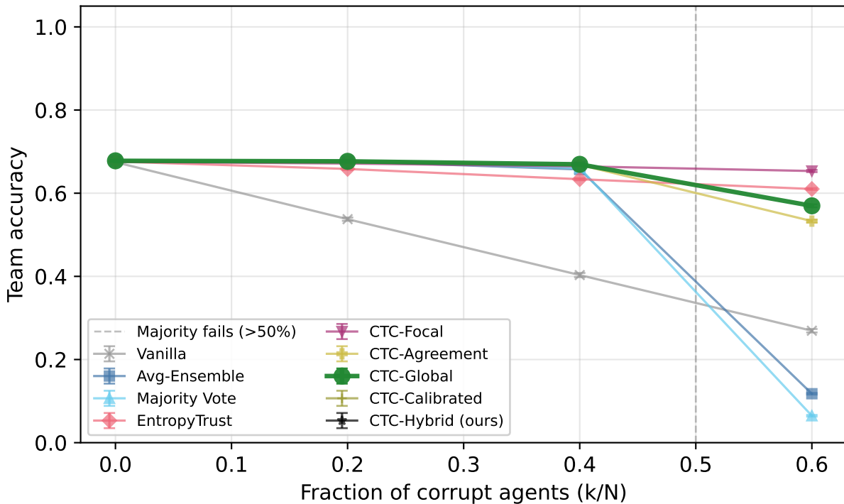
MMLU — Qwen2.5-7B-Instruct (overconfident, \alpha=0.1 )
