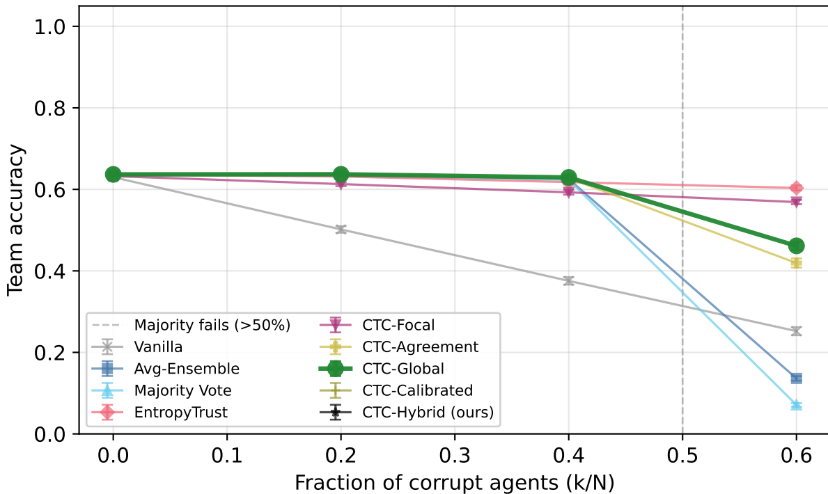
TRUTHFULQA — Phi-3.5-mini-instruct (overconfident, \alpha=0.1 )
