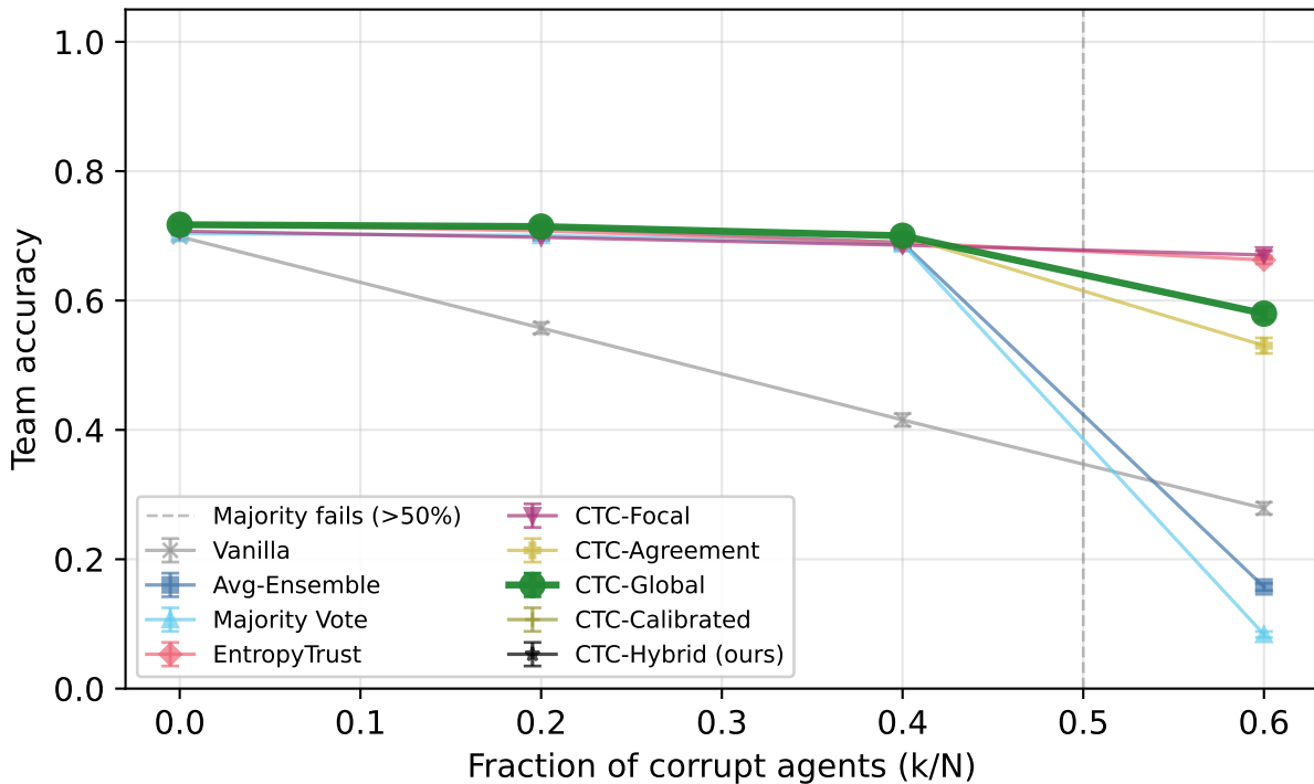
TRUTHFULQA — Qwen2.5-7B-Instruct (overconfident, \alpha=0.1 )
