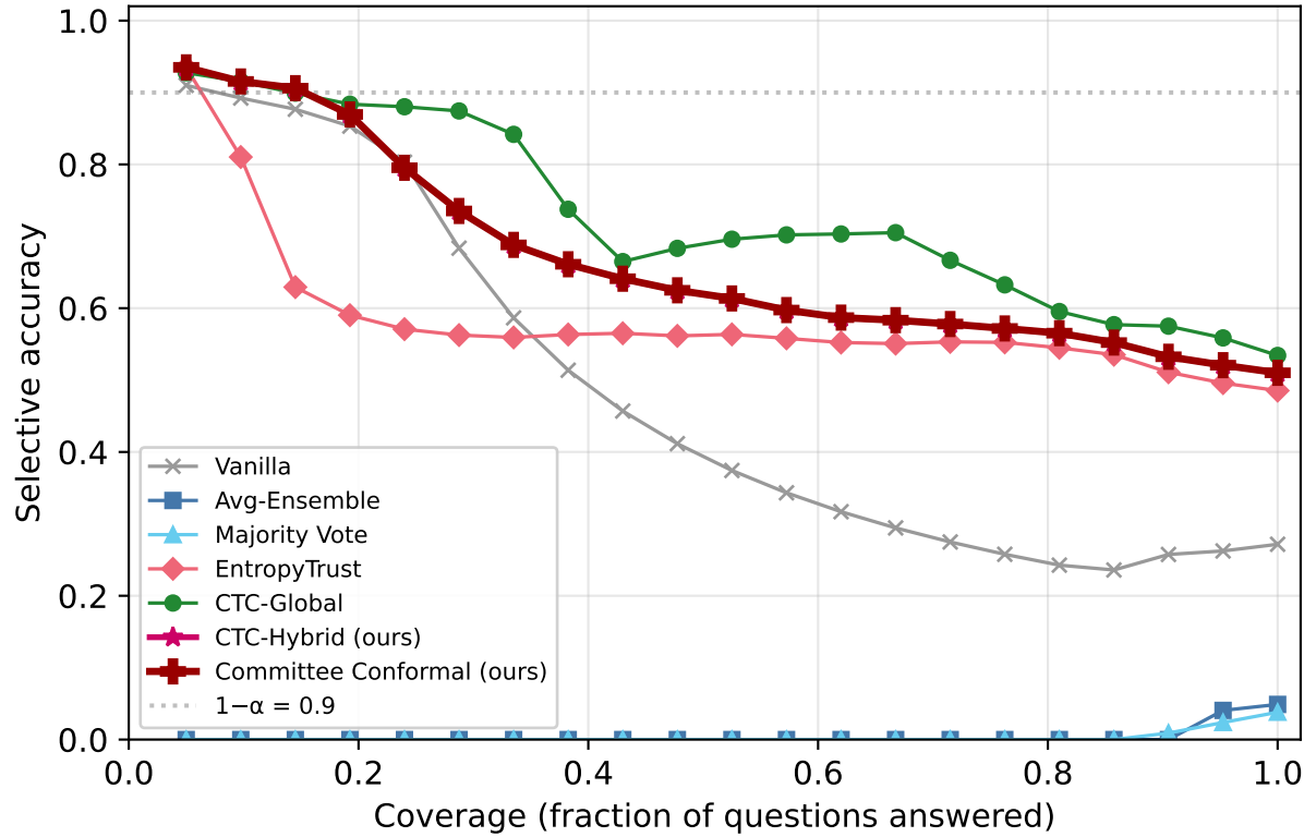
Risk-Coverage: ARC | Mistral-7B-Instruct-v0.3 | k=3/5 corrupt | overconfident_extreme
