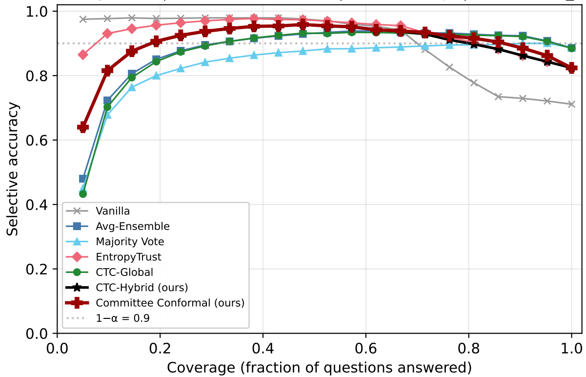
Risk-Coverage: ARC | Qwen2.5-7B-Instruct | k=1/5 corrupt | coordinated_extreme
