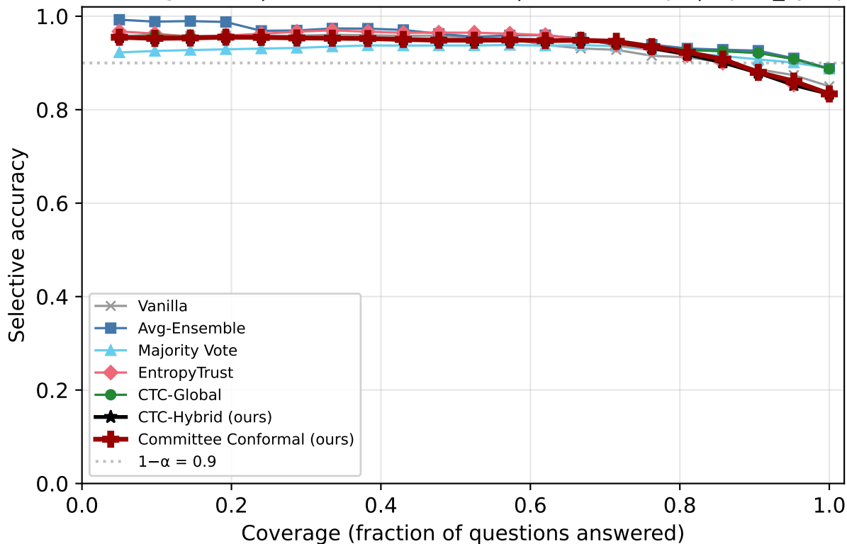
Risk-Coverage: ARC | Qwen2.5-7B-Instruct | k=1/5 corrupt | inject_sycophant
