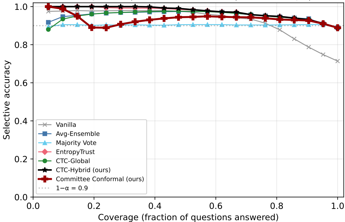
Risk-Coverage: ARC | Qwen2.5-7B-Instruct | k=1/5 corrupt | subtle
