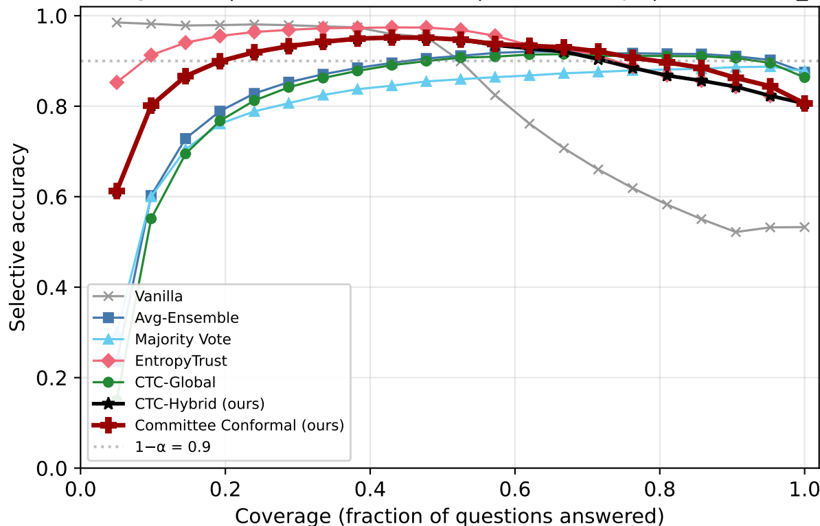
Risk-Coverage: ARC | Qwen2.5-7B-Instruct | k=2/5 corrupt | coordinated_extreme
