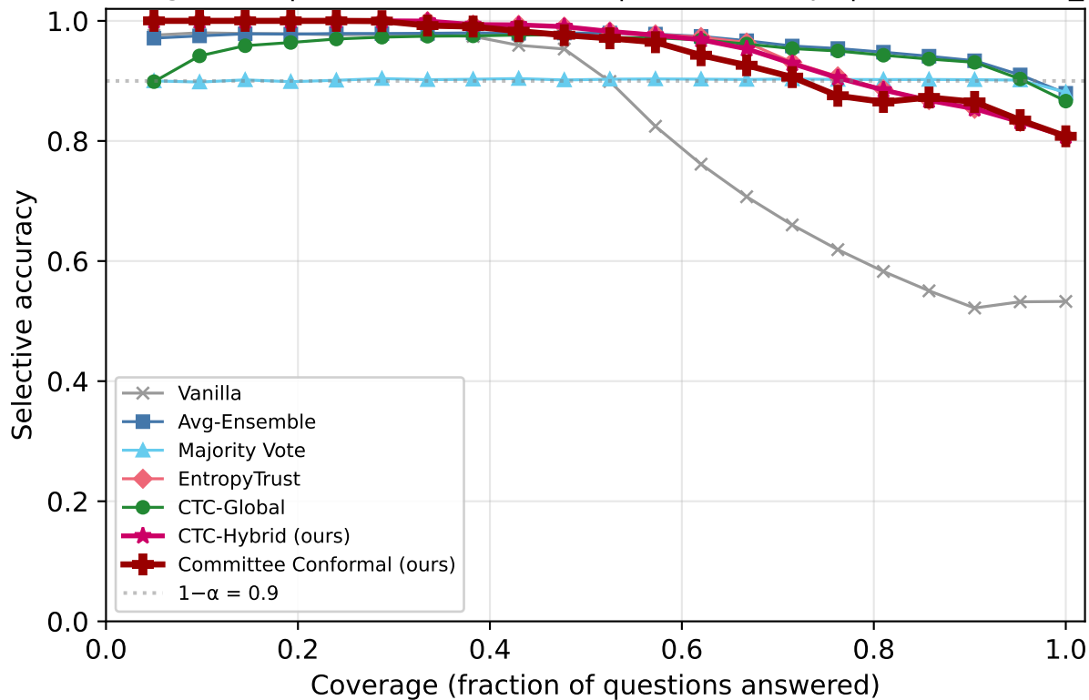
Risk-Coverage: ARC | Qwen2.5-7B-Instruct | k=2/5 corrupt | overconfident_extreme
