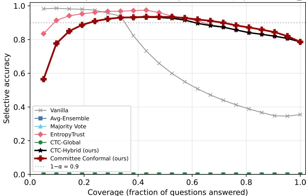
Risk-Coverage: ARC | Qwen2.5-7B-Instruct | k=3/5 corrupt | coordinated_extreme
