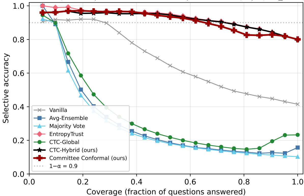
Risk-Coverage: ARC | Qwen2.5-7B-Instruct | k=3/5 corrupt | inject_deceptive
