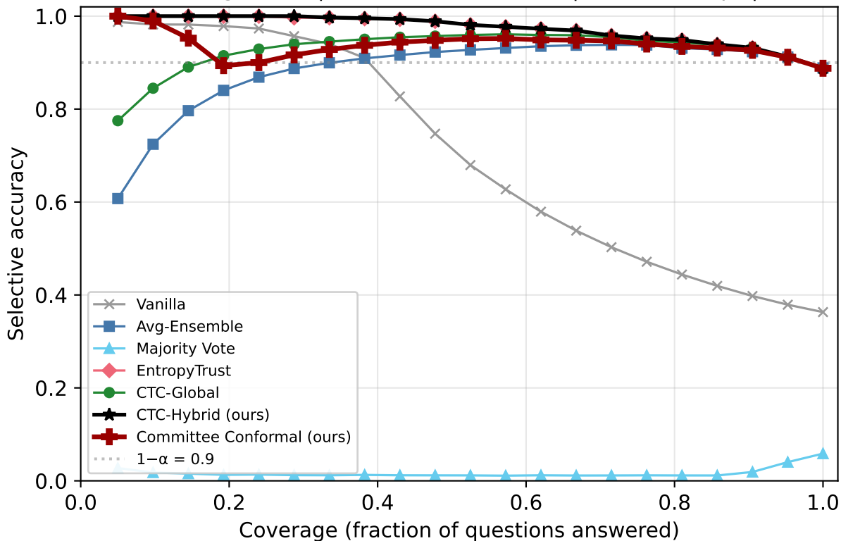
Risk-Coverage: ARC | Qwen2.5-7B-Instruct | k=3/5 corrupt | subtle
