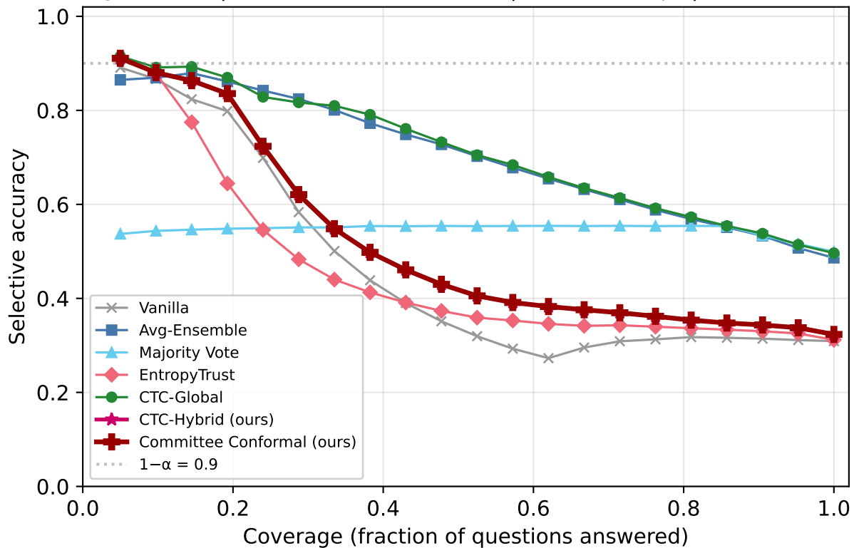
Risk-Coverage: MMLU | Mistral-7B-Instruct-v0.3 | k=2/5 corrupt | overconfident_extreme
