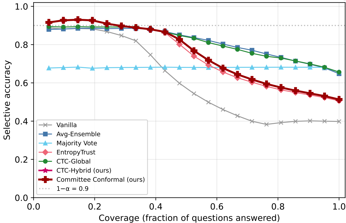
Risk-Coverage: MMLU | Phi-3.5-mini-instruct | k=2/5 corrupt | overconfident_extreme
