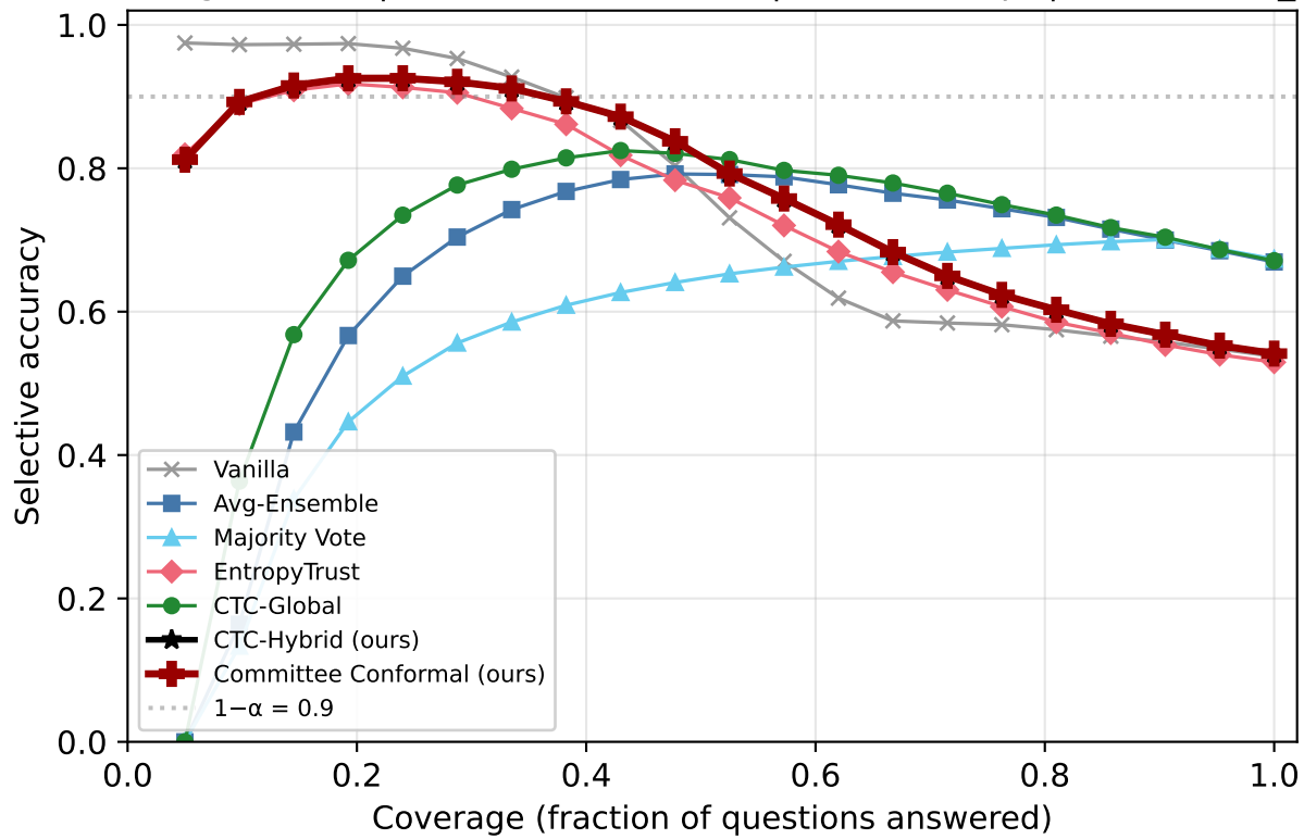
Risk-Coverage: MMLU | Qwen2.5-7B-Instruct | k=1/5 corrupt | coordinated_extreme
