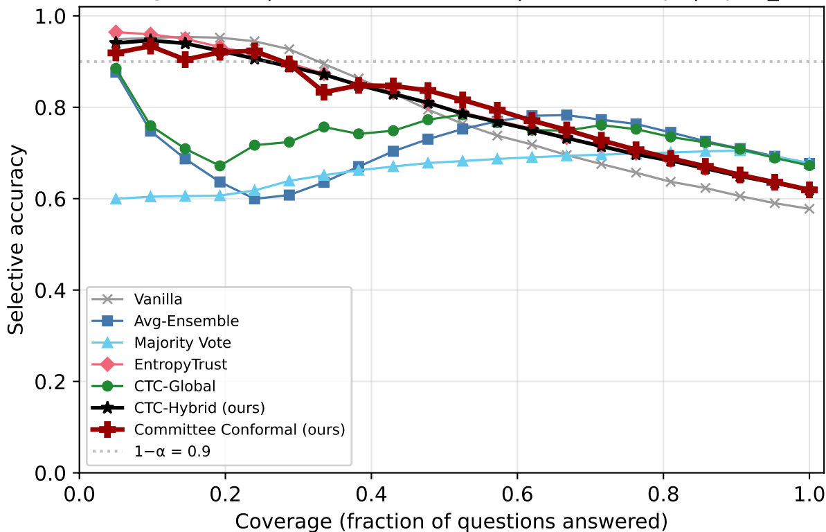
Risk-Coverage: MMLU | Qwen2.5-7B-Instruct | k=1/5 corrupt | inject_deceptive
