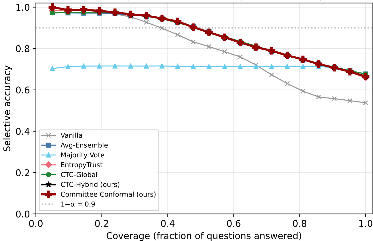
Risk-Coverage: MMLU | Qwen2.5-7B-Instruct | k=1/5 corrupt | overconfident
