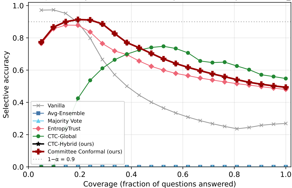
Risk-Coverage: MMLU | Qwen2.5-7B-Instruct | k=3/5 corrupt | coordinated_extreme
