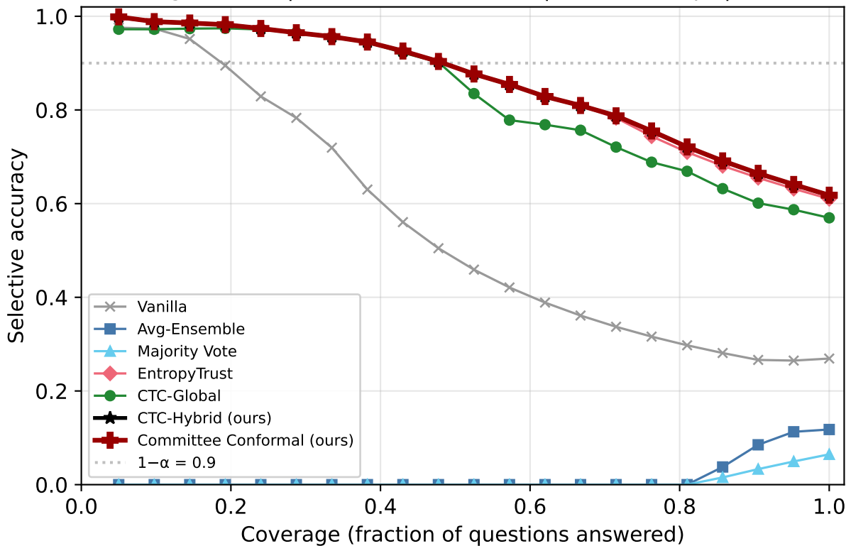
Risk-Coverage: MMLU | Qwen2.5-7B-Instruct | k=3/5 corrupt | overconfident
