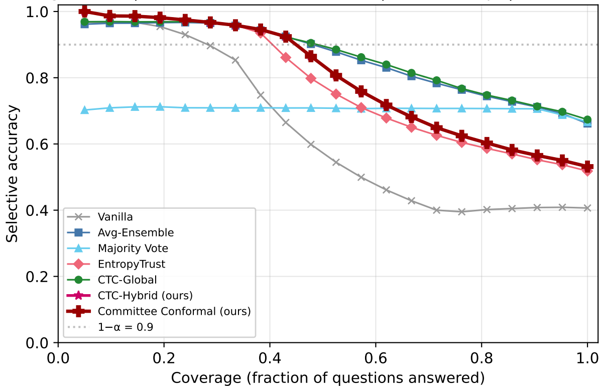
Risk-Coverage: MMLU | domain:Qwen2.5-7B-Instruct | k=2/5 corrupt | overconfident_extreme
