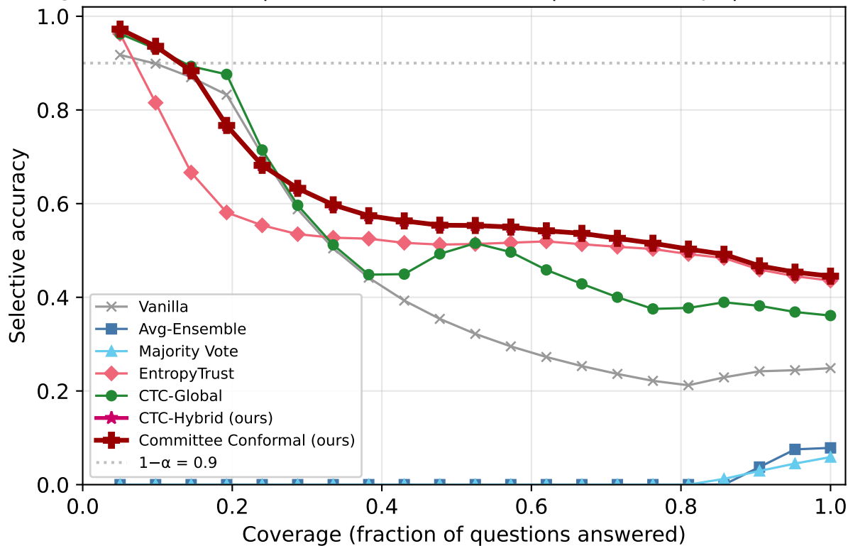
Risk-Coverage: TRUTHFULQA | Mistral-7B-Instruct-v0.3 | k=3/5 corrupt | overconfident_extreme
