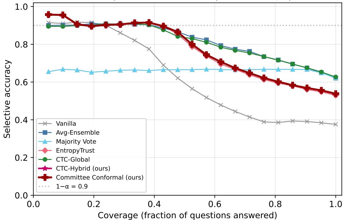
Risk-Coverage: TRUTHFULQA | Phi-3.5-mini-instruct | k=2/5 corrupt | overconfident_extreme
