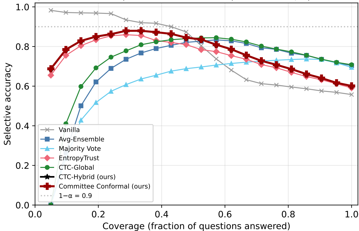
Risk-Coverage: TRUTHFULQA | Qwen2.5-7B-Instruct | k=1/5 corrupt | coordinated_extreme
