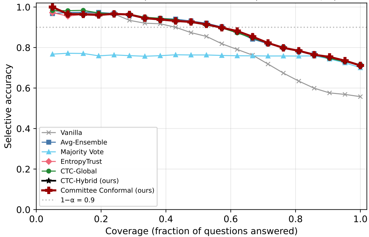
Risk-Coverage: TRUTHFULQA | Qwen2.5-7B-Instruct | k=1/5 corrupt | overconfident
