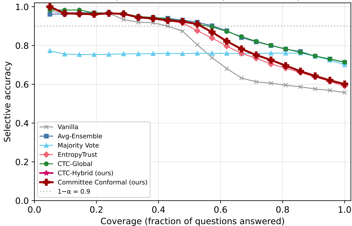
Risk-Coverage: TRUTHFULQA | Qwen2.5-7B-Instruct | k=1/5 corrupt | overconfident_extreme
