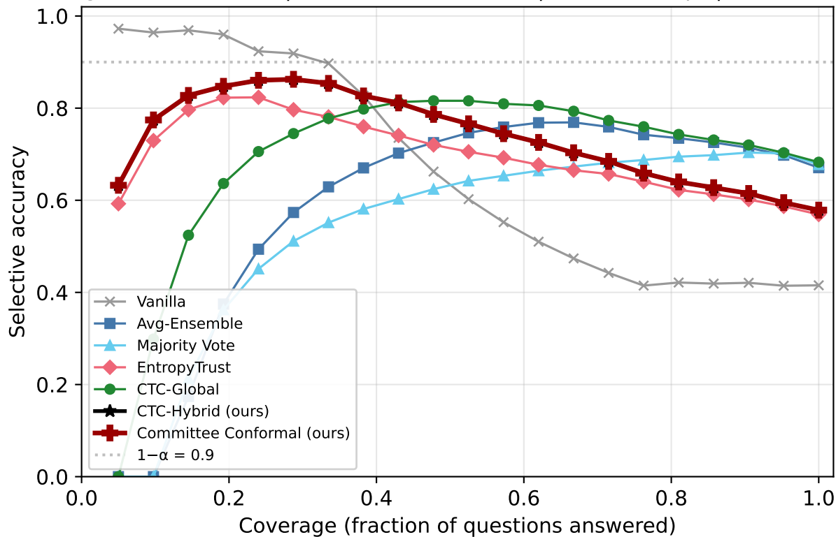
Risk-Coverage: TRUTHFULQA | Qwen2.5-7B-Instruct | k=2/5 corrupt | coordinated_extreme
