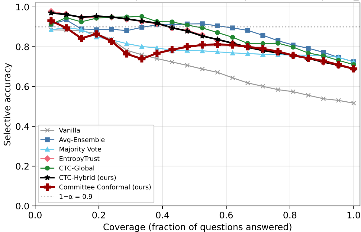
Risk-Coverage: TRUTHFULQA | Qwen2.5-7B-Instruct | k=2/5 corrupt | inject_deceptive
