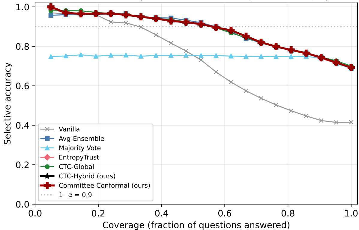
Risk-Coverage: TRUTHFULQA | Qwen2.5-7B-Instruct | k=2/5 corrupt | overconfident
