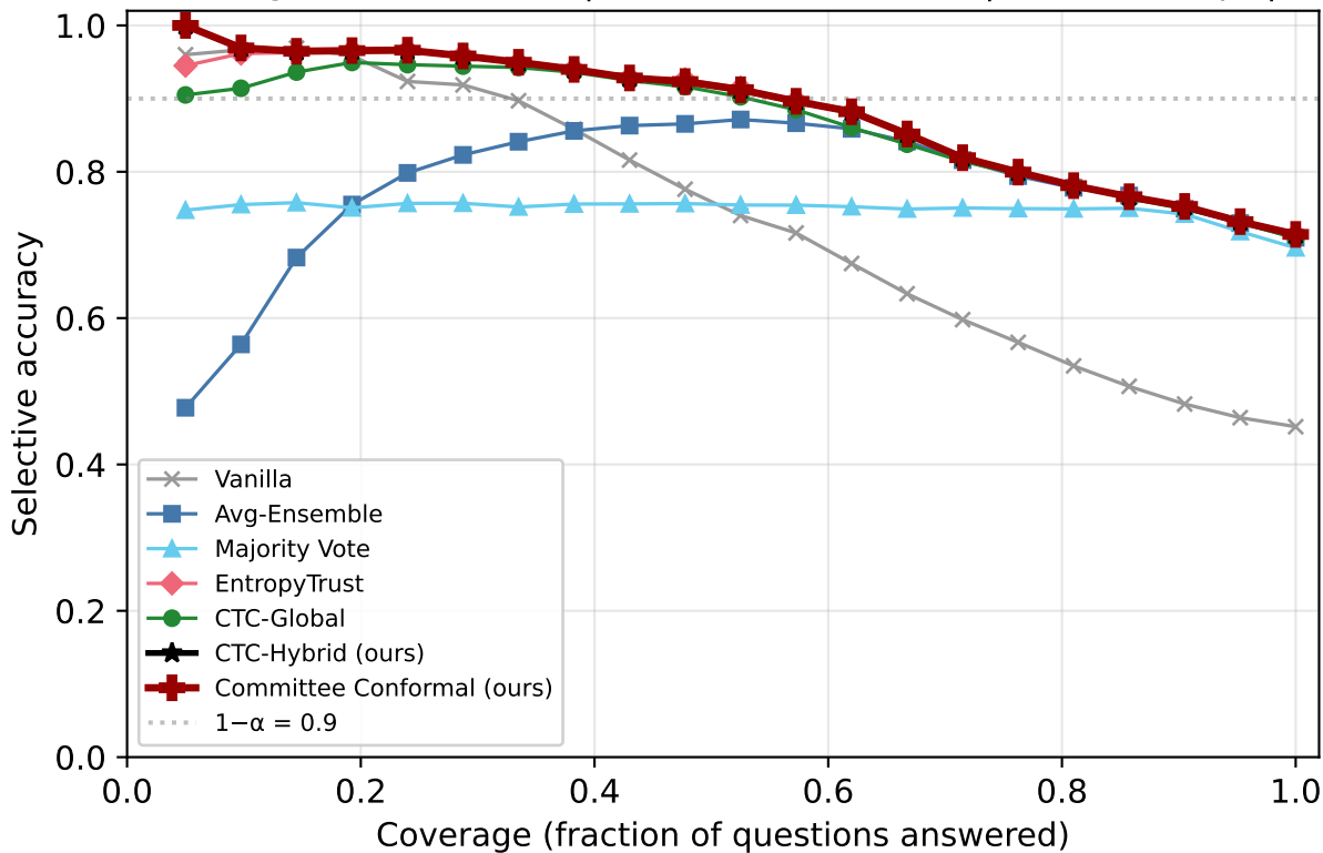
Risk-Coverage: TRUTHFULQA | Qwen2.5-7B-Instruct | k=2/5 corrupt | subtle
